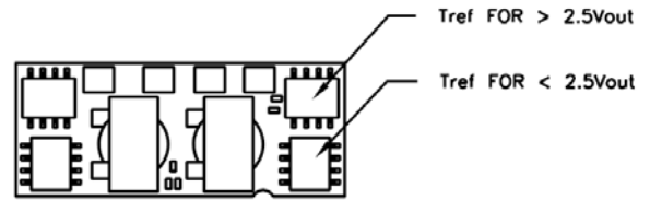
Figure 56. T_{ref} Temperature measurement location.
