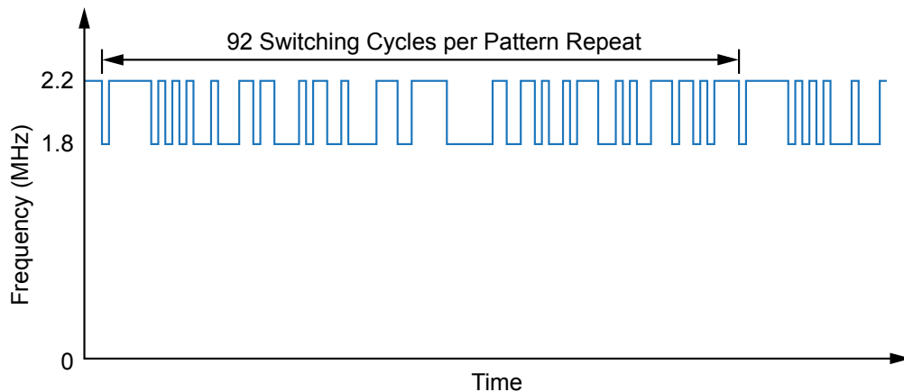
Figure 5: A8517 Dithering Scheme at 2 MHz ±10% (frequency jumps between 1.8 MHz and 2.2 MHz, as governed by a 46-bit pseudorandom pattern)
