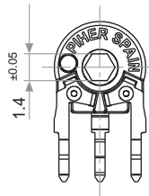
M Hexagonal thru hole
