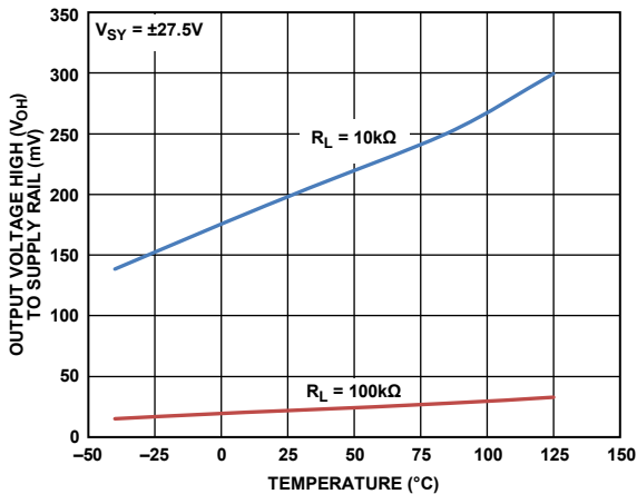
Figure 26. Output Voltage High ( V_{OH} ) to Supply Rail vs. Temperature, V_{SY} = \pm 27.5\text{V}
