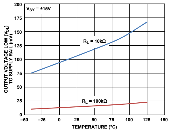
Figure 28. Output Voltage Low ( V_{OL} ) to Supply Rail vs. Temperature, V_{SY} = \pm 15\text{V}
