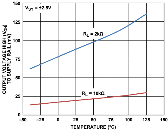
Figure 24. Output Voltage High ( V_{OH} ) to Supply Rail vs. Temperature, V_{SY} = \pm 2.5\text{V}
