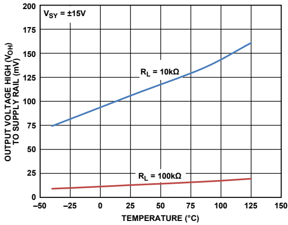
Figure 25. Output Voltage High ( V_{OH} ) to Supply Rail vs. Temperature, V_{SY} = \pm 15\text{V}
