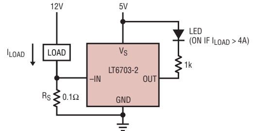
Low Side Current Sense Alarm
