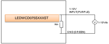
Implementation 2: DC input
