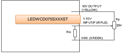
Implementation 1: Potentiometer control
