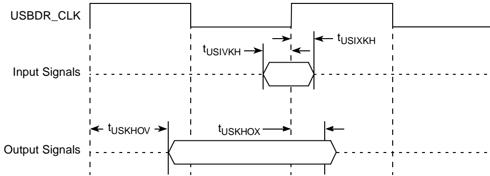
Figure 35. USB Signals
