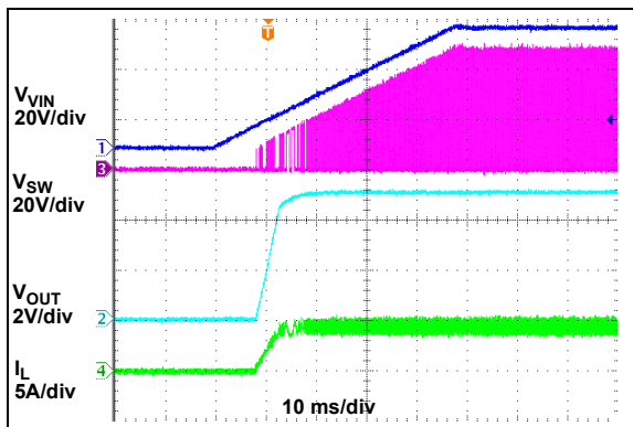
FIGURE 2-26: V_{VIN} Turn-On.
