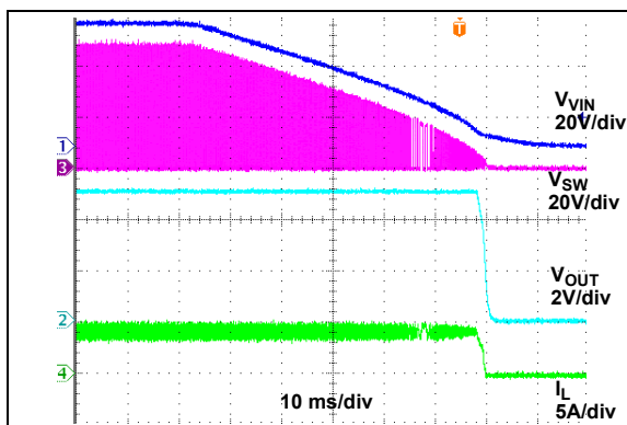
FIGURE 2-27: V_{VIN} Turn-Off.
