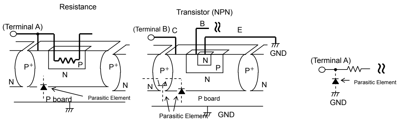
Fig.32 Simple Structure of Bipolar IC
