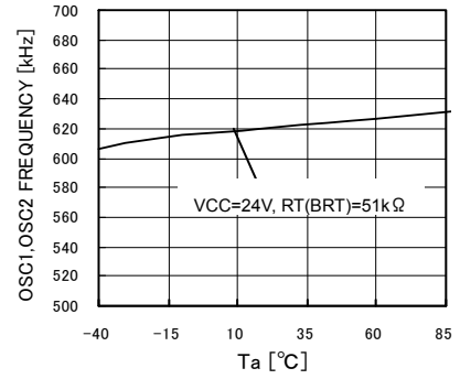
Fig.3 OSC1, OSC2 Temperature
