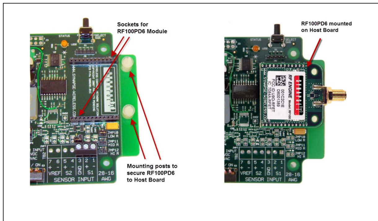
Host Board
