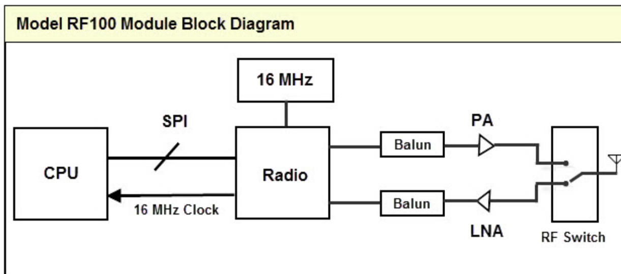
Figure 1.0 Block diagram showing the major subsystems comprising the RF100
