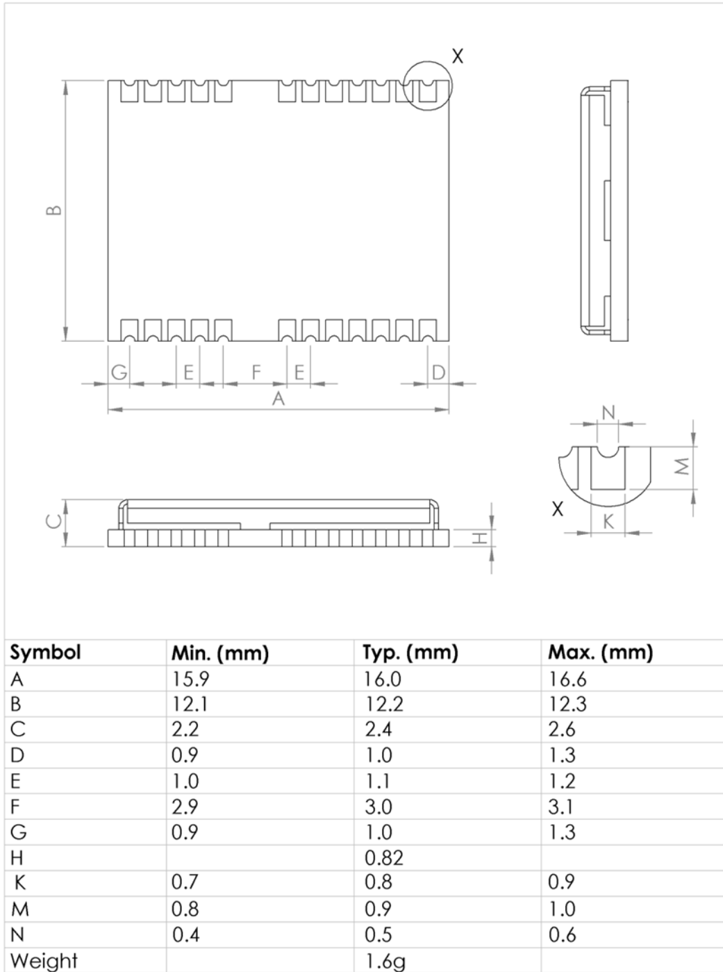
Figure 6: NEO dimensions
