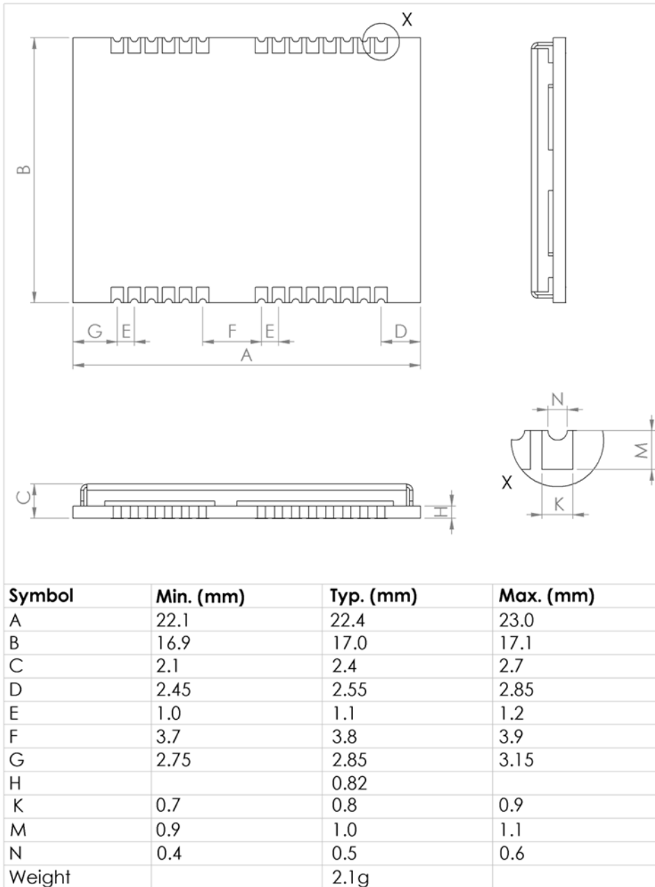
Figure 7: LEA dimensions
