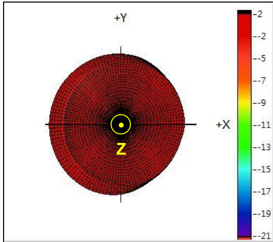
7-1-1. 3D Gain Pattern @ 1575.42 MHz (unit: dBi)
