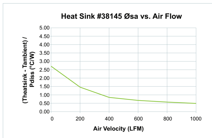
Figure 12. Heat sink to air thermal impedance part #38145 1.25" longitudinal fins
