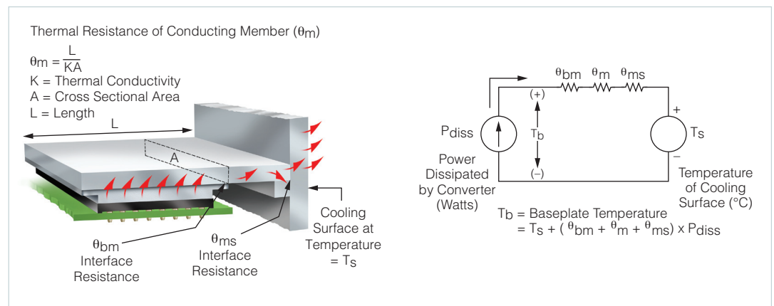
Figure 3. Interface thermal considerations
