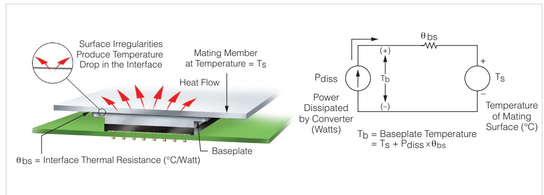
Figure 2. Baseplate thermal considerations
