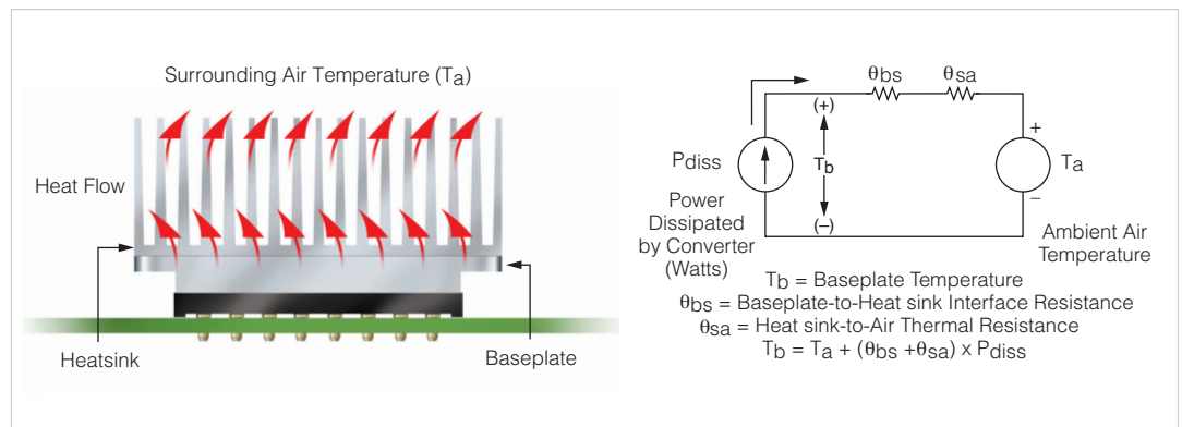
Figure 4. Heat sink thermal considerations
