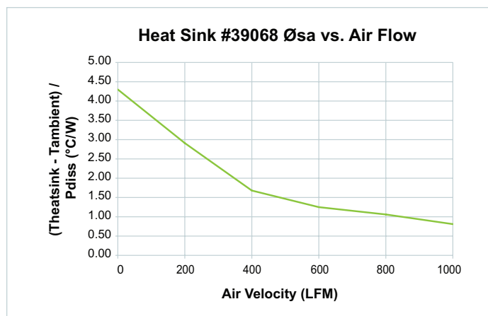
Figure 13. Heat sink to air thermal impedance part #39068 0.70" longitudinal fins
