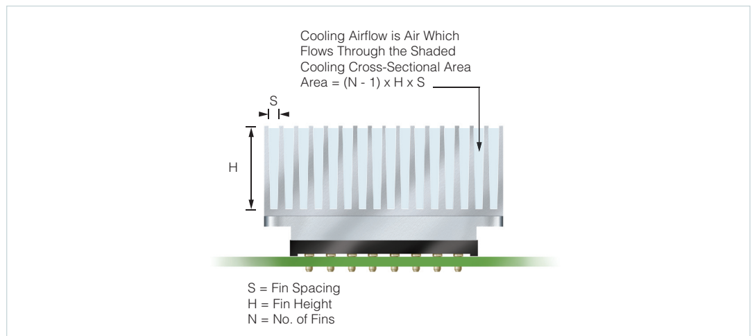
Figure 6. Heat sink cross section
