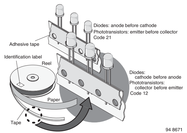
Fig. 21 - LED in Tape
