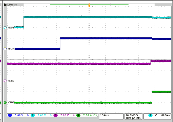
V_{VBUS} = 5\text{ V} V_{VBAT} = 3.2\text{ V} I_{CHG} = 2\text{ A} 图 10-3. Power-Up with Charge Enabled
