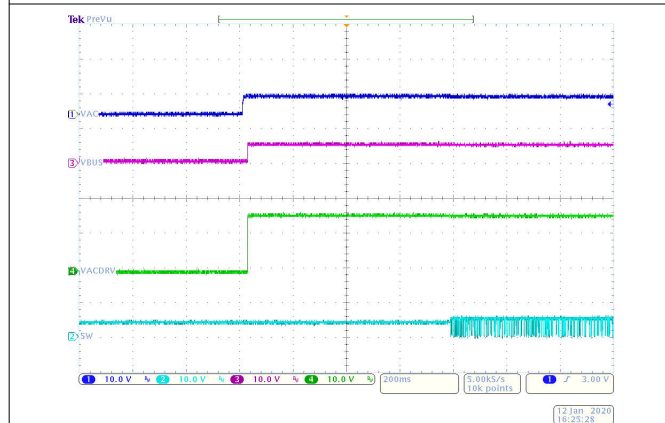
V_{VBUS} = 5\text{ V} V_{VBAT} = 3.2\text{ V} 图 10-4. OVPFET Turn-on during Power-Up
