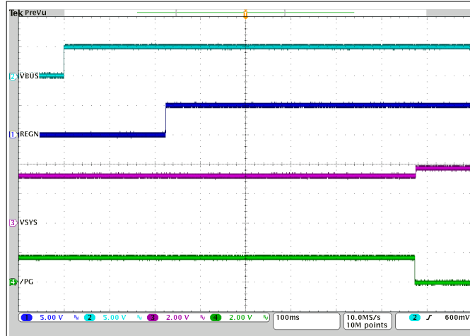
V_{VBUS} = 5\text{ V} V_{VBAT} = 3.2\text{ V} 图 10-2. Power-Up with Charge Disabled
