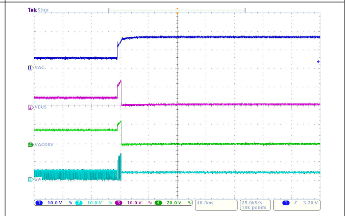
V_{VBUS} = 5\text{ V to }17\text{ V} V_{VBAT} = 3.2\text{ V} 图 10-5. OVPFET Turn-off during Input OVP
