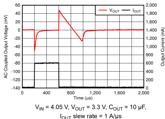
Figure 8-9. I_{OUT} Transient From 1 mA to 600 mA
