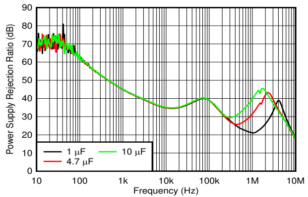
V_{OUT} = 3.3\text{ V} , I_{OUT} = 1\text{ A} Figure 6-26. PSRR vs C_{OUT}
