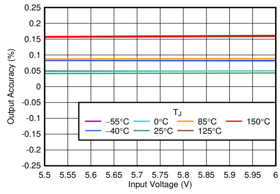
Figure 6-2. Output Accuracy vs V_{IN}
