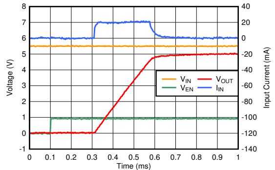
V_{IN} = 5.5\text{ V} , C_{IN} = 0\ \mu\text{F} , C_{OUT} = 1\ \mu\text{F} , V_{OUT} = 5.0\text{ V} , I_{OUT} = 0\text{ mA} Figure 6-28. Start-Up Inrush Current With C_{OUT} = 1\ \mu\text{F}
